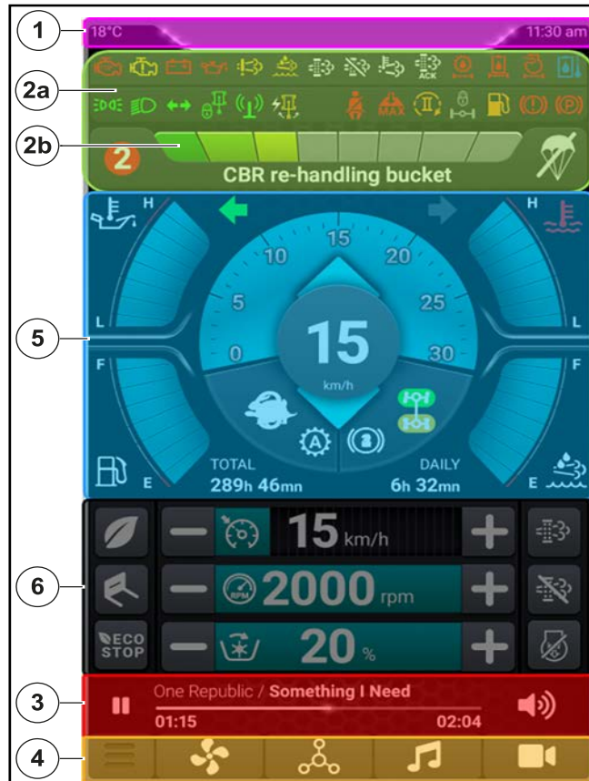
Figure 78: Zone du HMI
