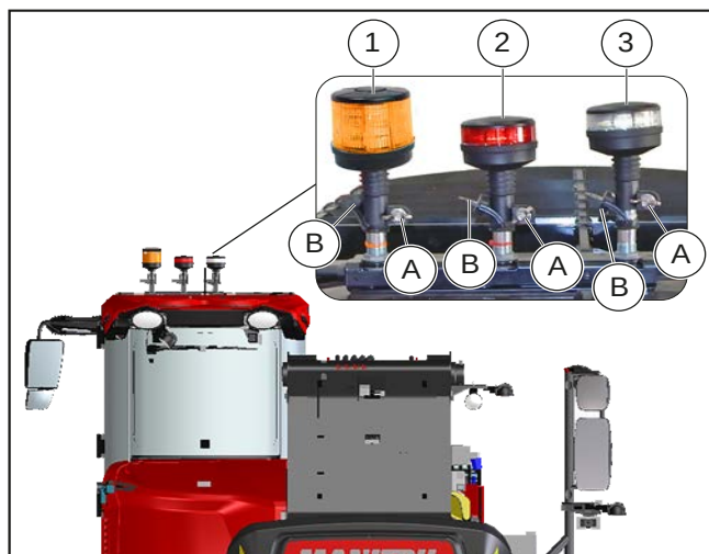
Figure 65: Phares et gyrophare
